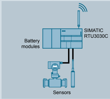
Self-sufficient measuring station
