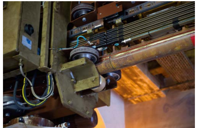
IWLAN antennas provide continuous wireless communication even at segment transitions. The Rapid Roaming function provides transfer times of less than 32 milliseconds between access points
