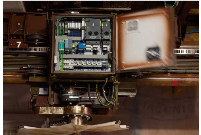
Control box installed on gondola including fail-safe SIMATIC PLC, fail-safe frequency converters (right) and IWLAN client Scalance W740 (top) for wireless, fail-safe PROFINET communication
